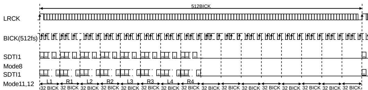
Figure 30. Mode 20/23/24 Timing
