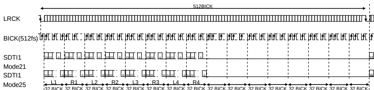
Figure 31. Mode 21/25 Timing
