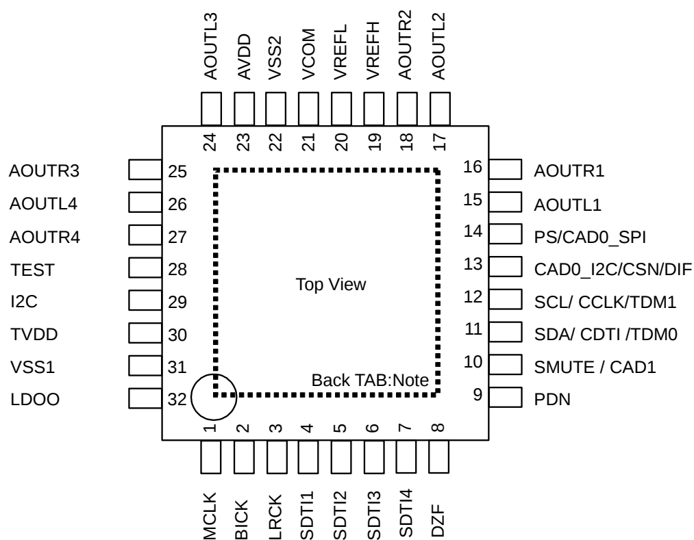
Figure 2. Pin Configurations
