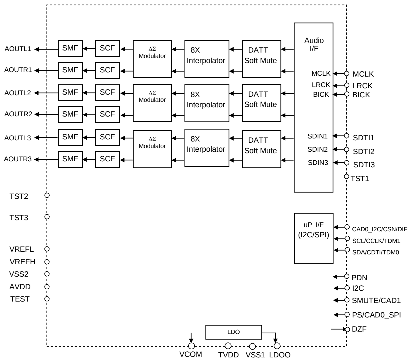
Figure 1. Block Diagram
