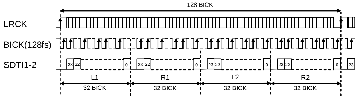
Figure 19. Mode 10 Timing
