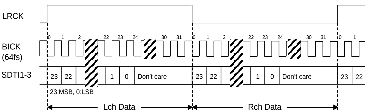
Figure 13. Mode 2 Timing
