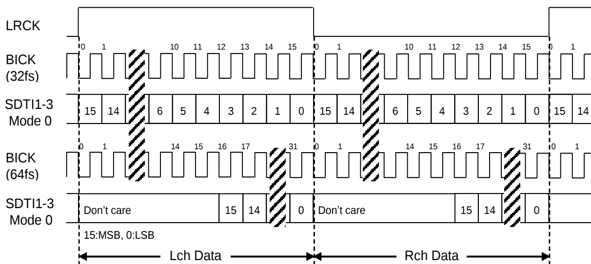
Figure 11. Mode 0 Timing
