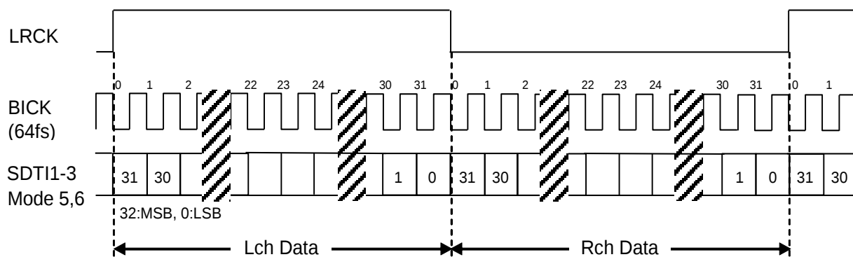
Figure 15. Mode 5/6 Timing
