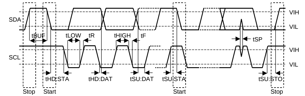
Figure 9. I²C Bus mode Timing
