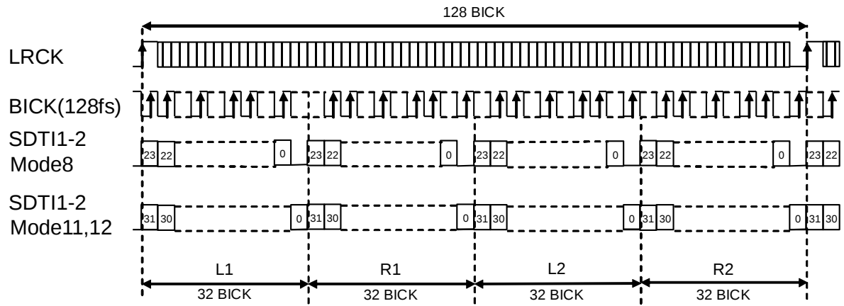
Figure 17. Mode 8/11/12 Timing
