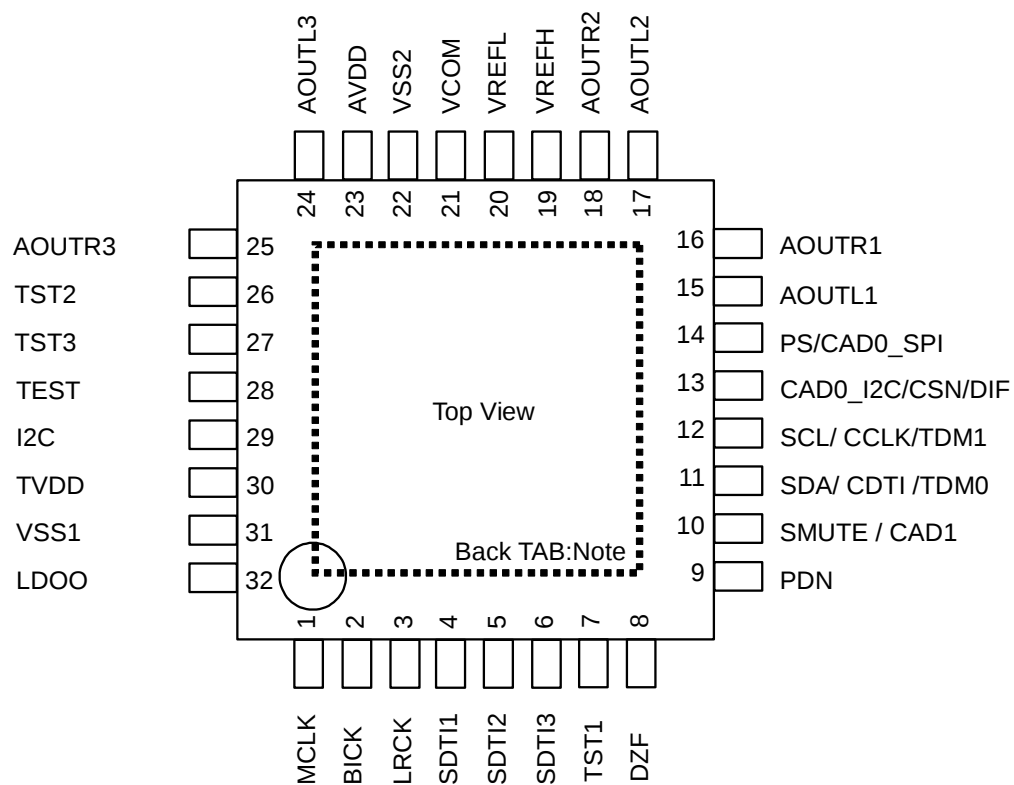
Figure 2. Pin Configurations
