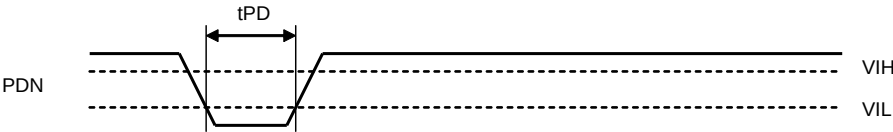
Figure 10. Power-down & Reset Timing
