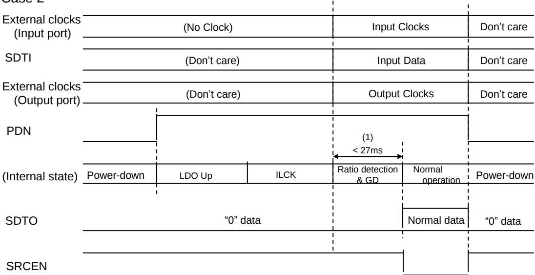
Figure 44. System Reset 2
