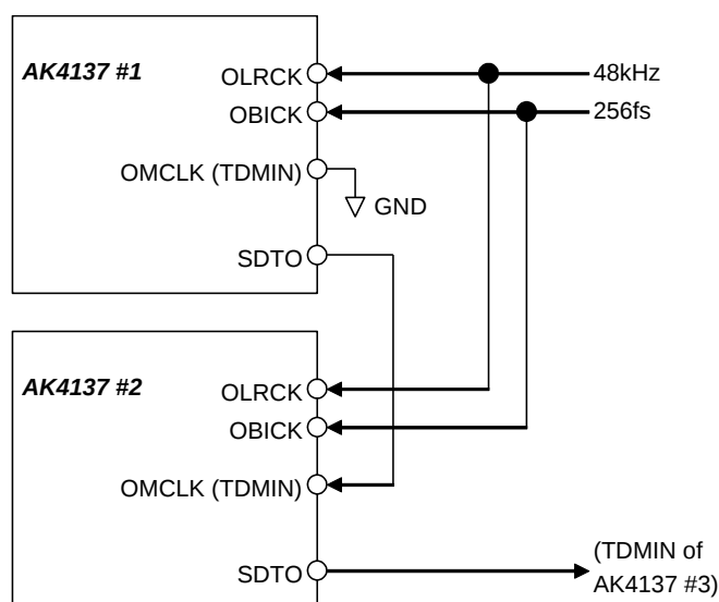
Figure 37. Cascade Connection Example
