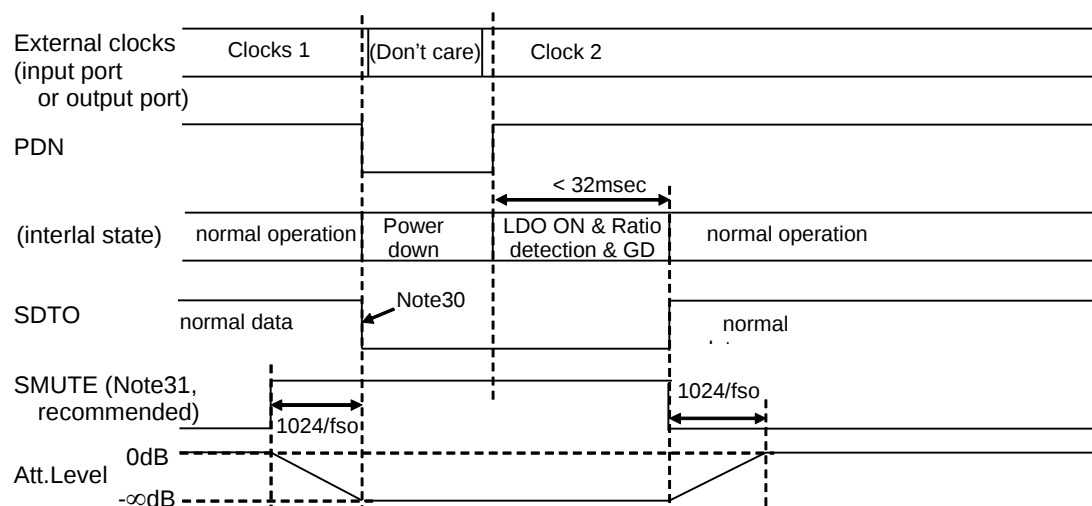
Figure 45. Sequence of Changing Clocks (Parallel Control Mode, PSN pin= "H")
