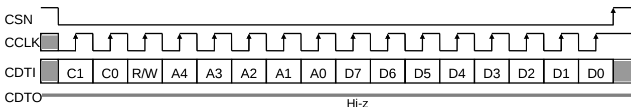
Figure 48. Write Operation
