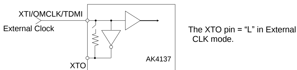
Figure 21. External Clock (OMCLK) Mode
