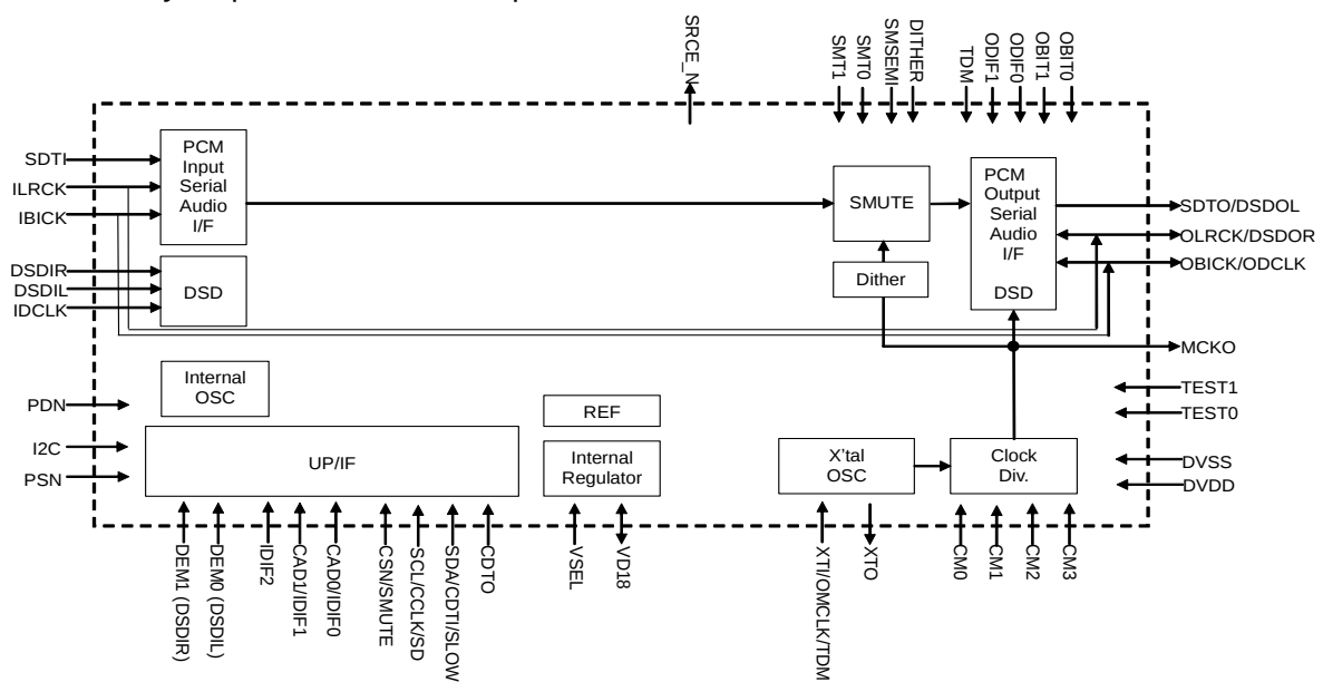
Figure 17. BYPASS Mode Master (PCMIN→PCMOUT)
