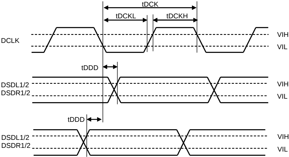
Figure 10. Audio Serial Interface Timing
