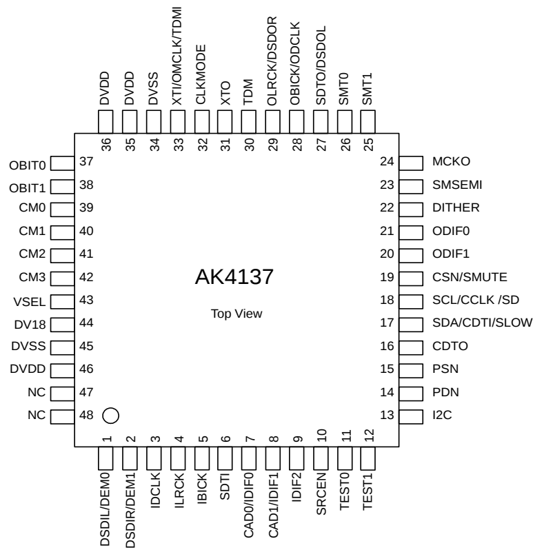
Figure 2. Pin Layout
