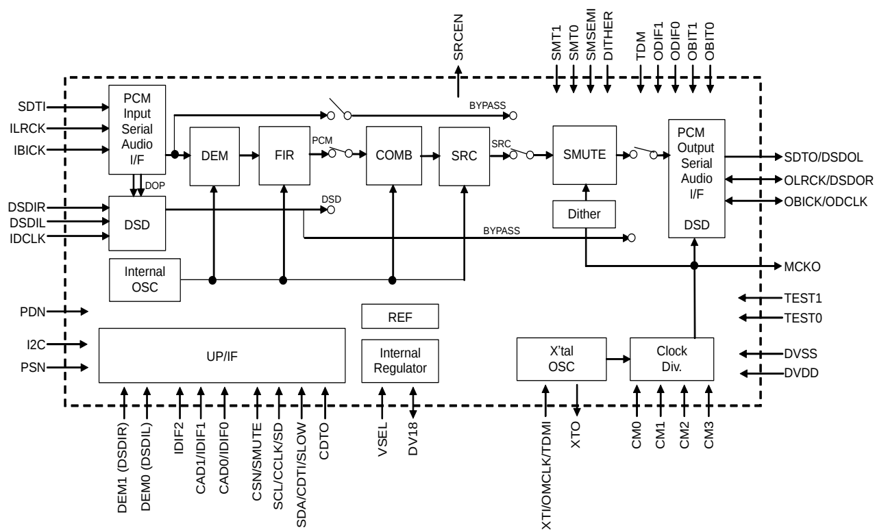
Figure 1. Block Diagram
