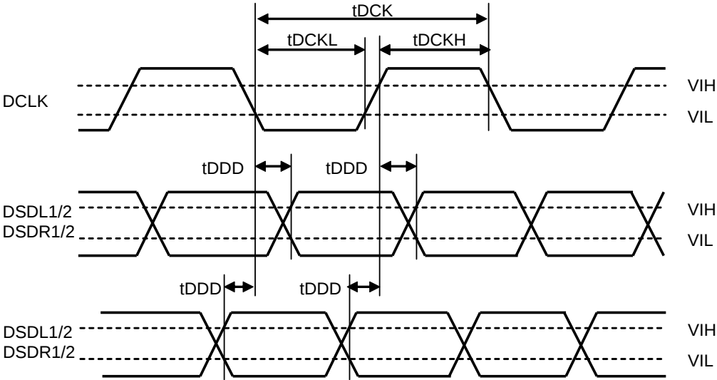
Figure 11. Audio Serial Interface Timing
