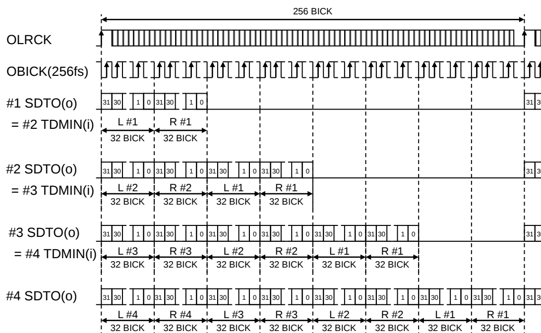
Figure 38. TDM Cascade
