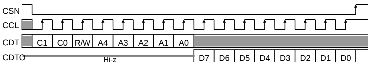
Figure 49. Read Operation
