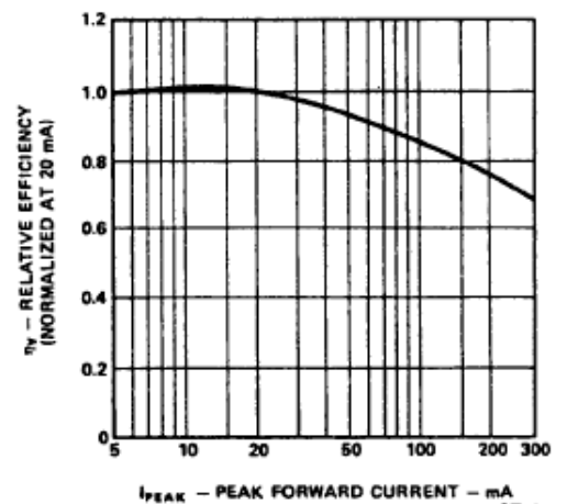
Figure 6. Relative Efficiency vs. Peak Forward Current
