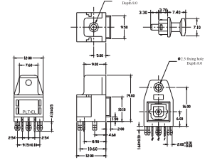
Package Dimensions
