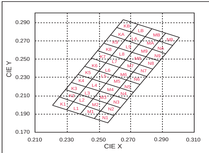
Chromaticity Diagram
