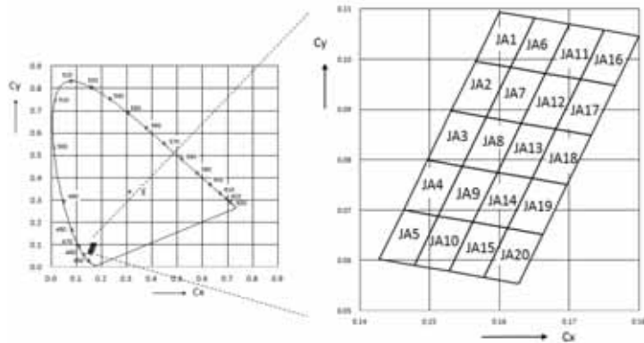
Bin Range of Chromaticity Coordinates Specifications
