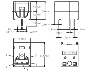
Package Dimensions
