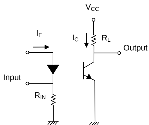
Figure 8. Switching Time Test Circuit & Waveforms
