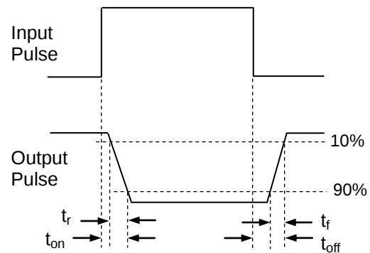
Figure 8. Switching Time Test Circuit & Waveforms
