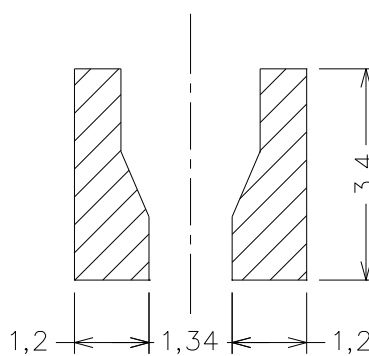
Soldering patterns
