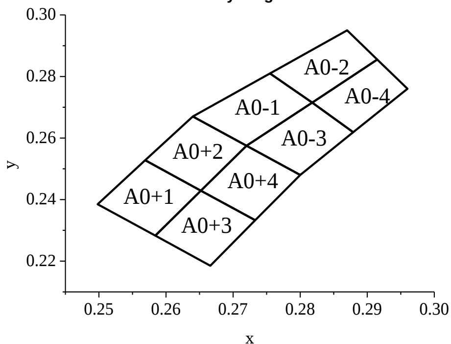
The C.I.E. 1931 Chromaticity Diagram
