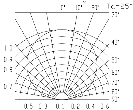
Radiation Diagram
