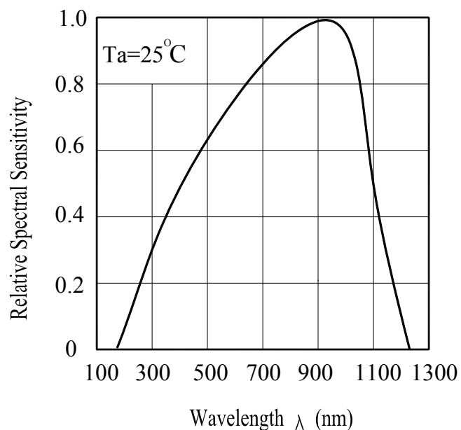
Spectral Sensitivity
