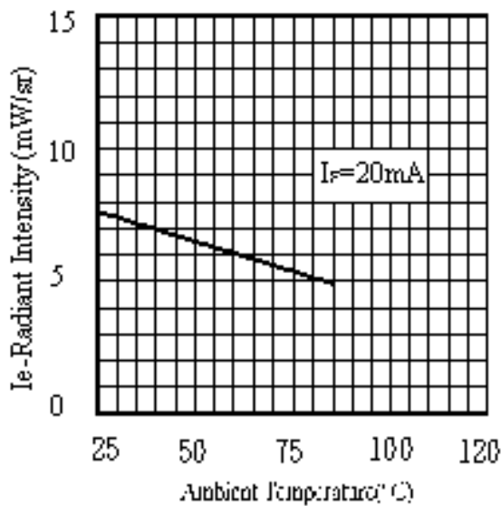
Ie-Radiant Intensity vs. Ambient Temperature
