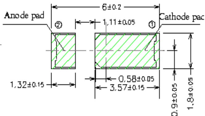
Soldering patterns
