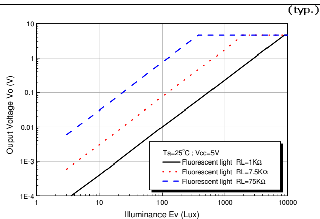
Fig.2 Output Voltage vs. Illuminance
