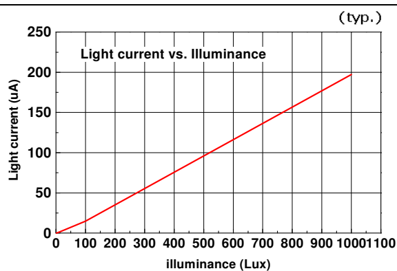
Fig.6 (LED) Light Current vs. Illuminance
