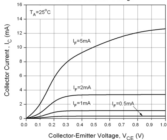
Figure 6. Collector Current vs Collector-Emitter Voltage
