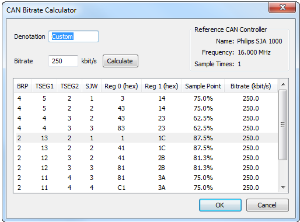
Figure 5.15: The CAN bitrate calculator
