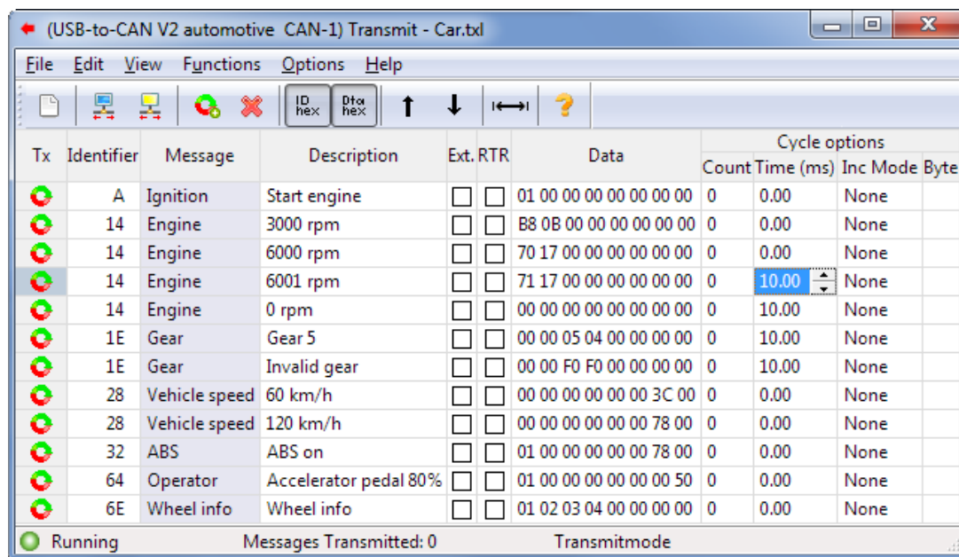
Figure 5.37: Edit mode of the cells
