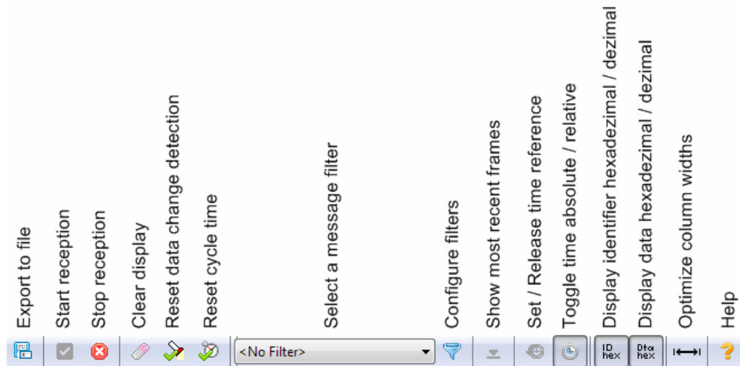
Figure 5.30: Toolbar of the Receive module
