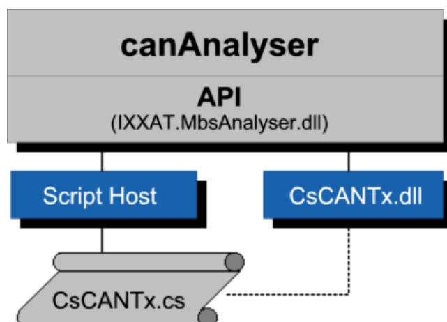
Figure 5.66: Integration of "C# CAN Tx" sample as assembly DLL and via Script Host.
