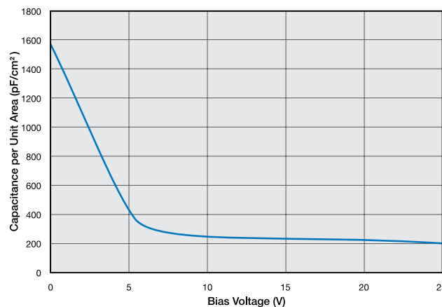
Typical Capacitance per Unit Area vs. Bias Voltage
