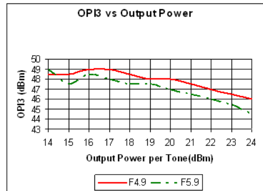
Figure 5 OIP3
