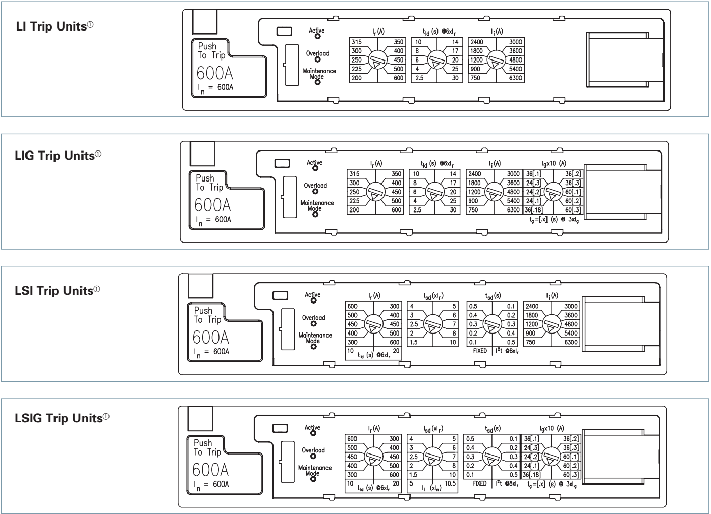
Typical Trip Unit Labeling and Adjustment Positions for the Sentron Sensitrip Circuit Breaker.
