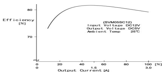
Efficiency Curve
