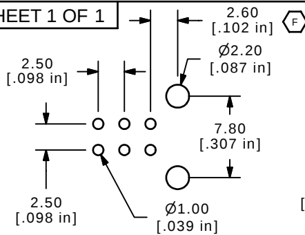
P.C. MOUNTING
