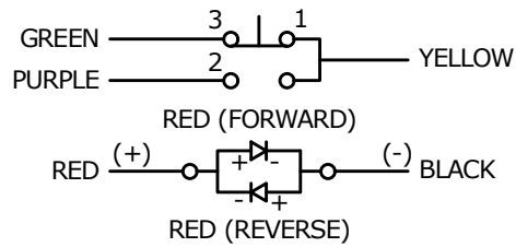
SCHEMATIC ON - ON - SPDT ILLUMINATED
