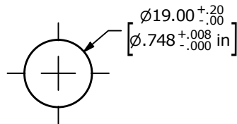
RECOMMENDED PANEL CUTOUT MAX. PANEL THICKNESS 10.0 [.39 in]
