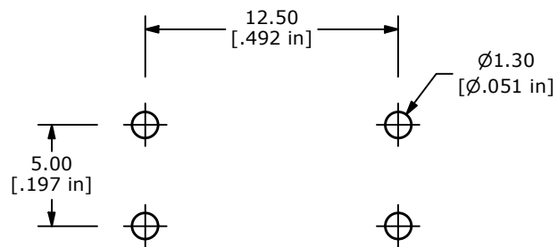
P.C.B. MOUNTING
