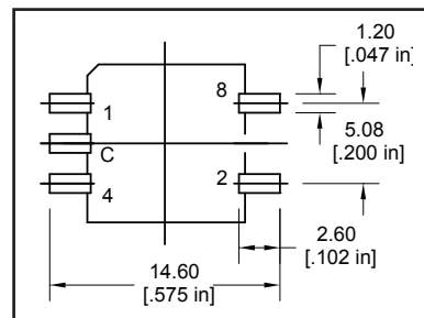
VERTICAL S2 PCB LAYOUT
