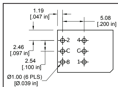
RT ANGLE R1 PCB LAYOUT
