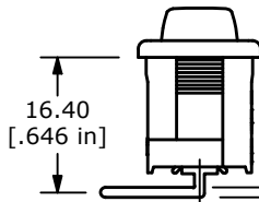
"L" TERMINAL (LEFT ANGLE) (TERMINALS BENT AWAY FROM LOGO SIDE)
