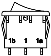
"L" TERMINAL (LEFT ANGLE) (TERMINALS BENT AWAY FROM LOGO SIDE)
