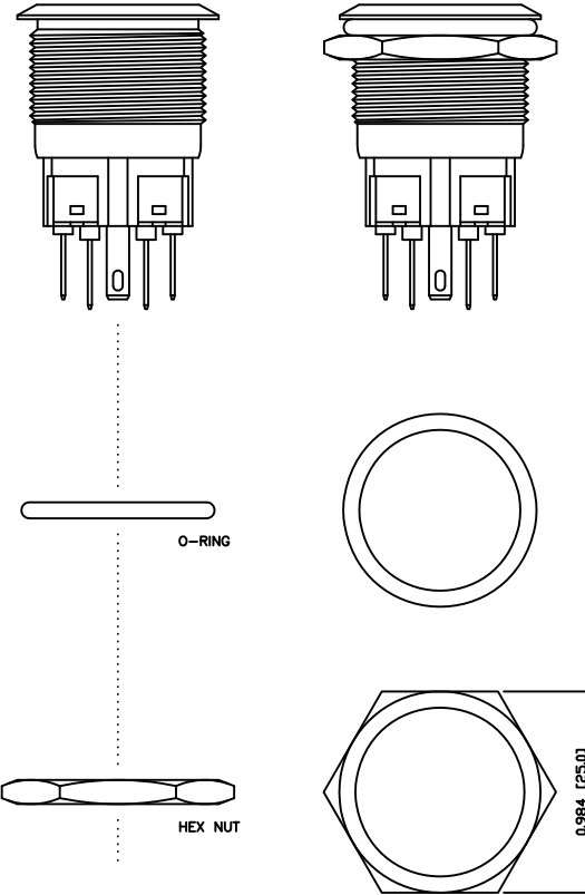
EXPLODED VIEW
