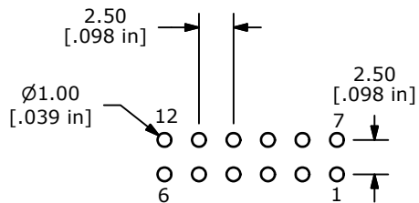
P.C. MOUNTING
