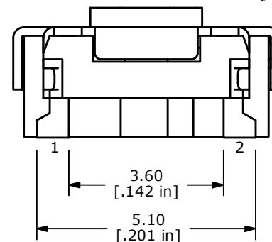
CHASSIS SOLDER TAB
