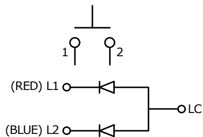
LED SCHEMATIC
