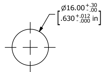
PANEL MOUNTING
