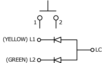
LED SCHEMATIC
