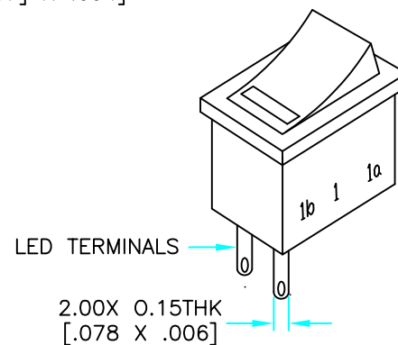
ORTHOGRAPHIC PROJECTION FOR CLARITY ONLY
