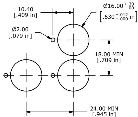
PANEL MOUNTING
