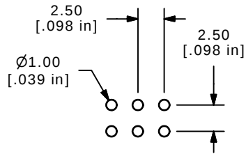
P.C. MOUNTING
