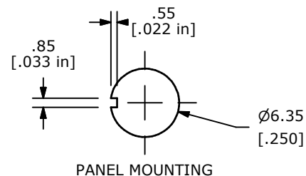
PANEL MOUNTING
