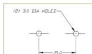
PANEL MOUNT
