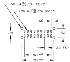
P.C. MOUNTING
