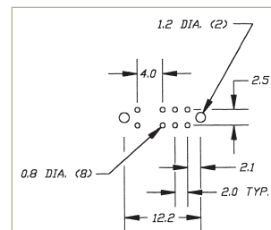
P.C. MOUNTING
