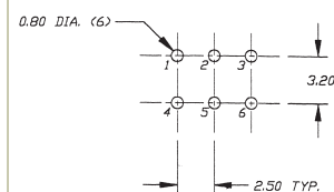
P.C. MOUNTING
