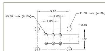
P.C. MOUNTING
