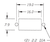
P.C. MOUNTING
