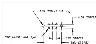
P.C. MOUNTING
