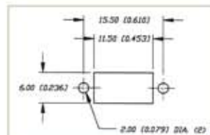
PANEL MOUNT
