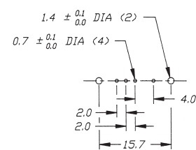
P.C. MOUNTING
