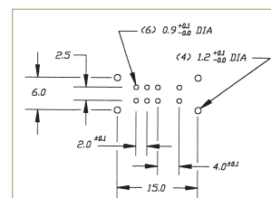
P.C. MOUNTING
