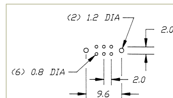
P.C. MOUNTING
