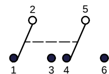
▲ CIRCUIT: DPDT
