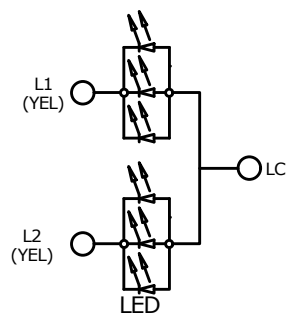
LED SCHEMATIC
