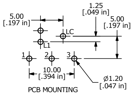
PCB MOUNTING
