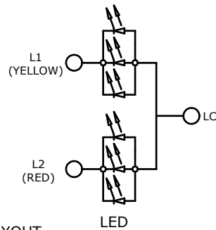
CIRCUIT LAYOUT
