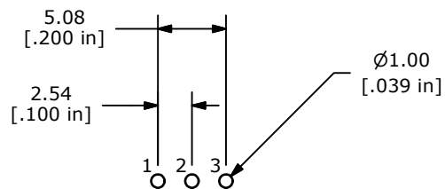
PCB LAYOUT
