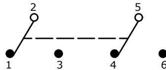
CIRCUIT: DPDT
