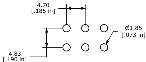
PCB LAYOUT
