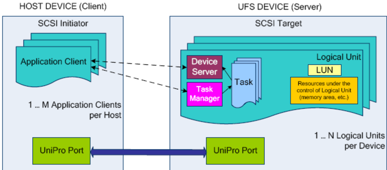
Figure 4-1- UFS SCSI Domain
