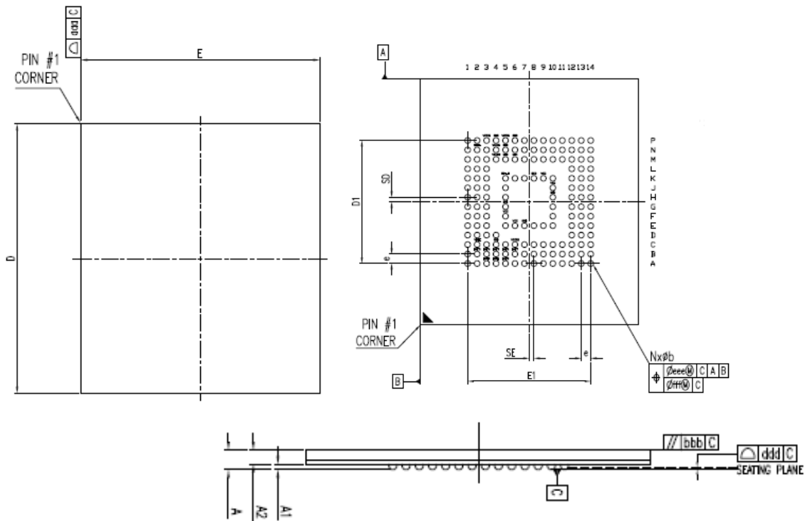
Figure 2 – Package Dimensions
