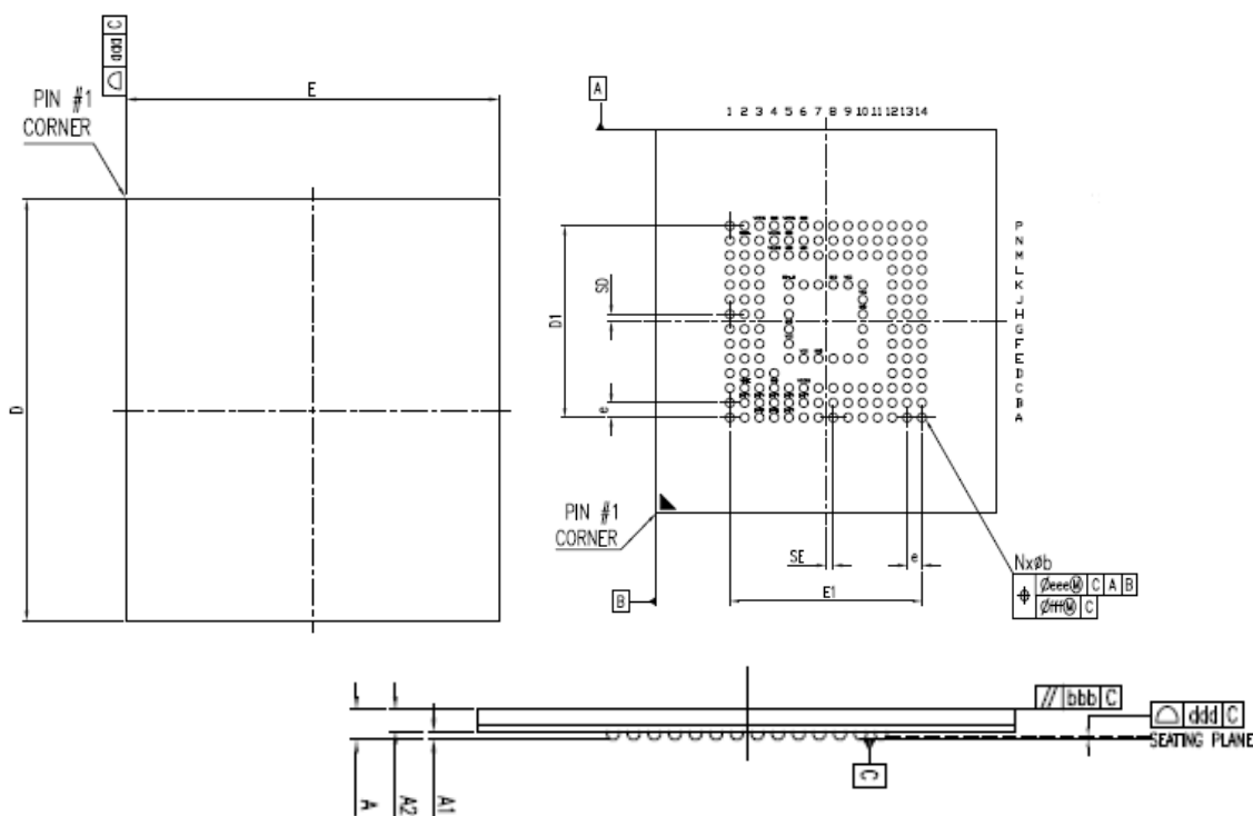
Figure 2 – Package Dimensions
