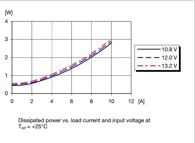
Power Dissipation
