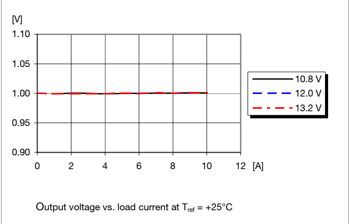
Output Characteristics
