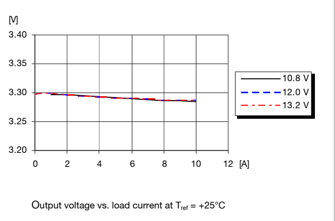
Output Characteristics
