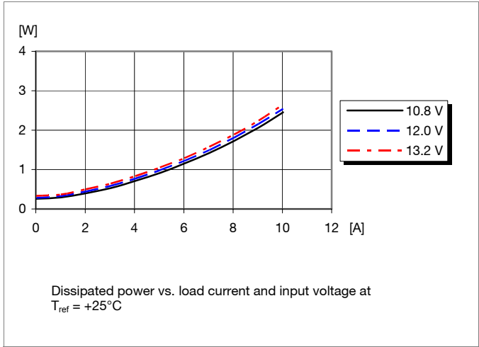
Power Dissipation
