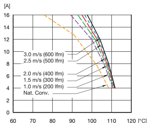
Available load current vs. ambient air temperature and airflow at V_{in} = 5\text{ V} . See conditions on page 27.
