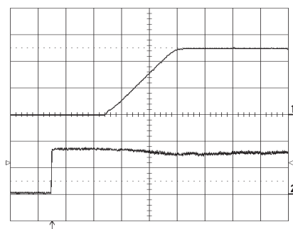
Start-up at I_O = 16\text{ A} resistive load at T_{ref} = +25\text{ }^{\circ}\text{C} , V_{in} = 3.3\text{ V} . Start enabled by connecting V_{in} . Top trace: output voltage (1 V/div.). Bottom trace: input voltage (2 V/div.). Time scale: 2 ms/div.
