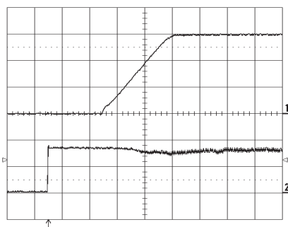
Start-up at I_O = 16\text{ A} resistive load at T_{ref} = +25\text{ }^{\circ}\text{C} , V_{in} = 3.3\text{ V} . Start enabled by connecting V_{in} . Top trace: output voltage (0.5 V/div.). Bottom trace: input voltage (2 V/div.). Time scale: 2 ms/div.
