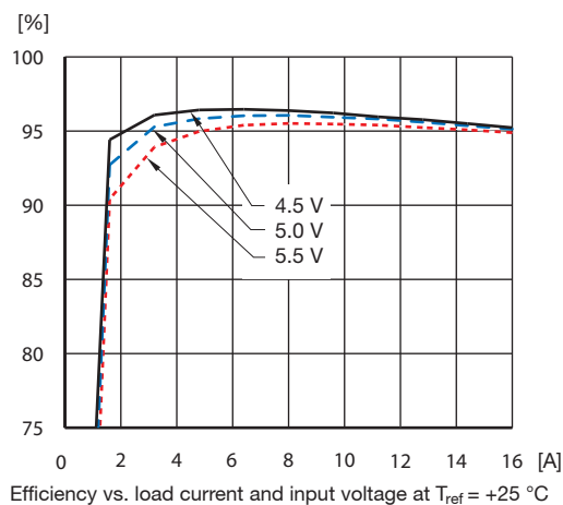
Efficiency vs. load current and input voltage at T_{ref} = +25\text{ }^{\circ}\text{C}
