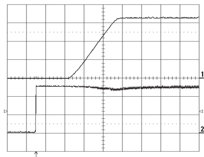
Start-up at I_O = 16\text{ A} resistive load at T_{ref} = +25\text{ }^{\circ}\text{C} , V_{in} = 5\text{ V} . Start enabled by connecting V_{in} . Top trace: output voltage (1 V/div.). Bottom trace: input voltage (2 V/div.). Time scale: 2 ms/div.
