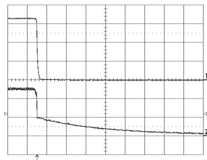
Turn-off at I_O = 16\text{ A} resistive load at T_{ref} = +25\text{ }^{\circ}\text{C} , V_{in} = 5\text{ V} . Turn-off enabled by disconnecting V_{in} . Top trace: output voltage (1 V/div.). Bottom trace: input voltage (2 V/div.). Time scale: 2 ms/div.
